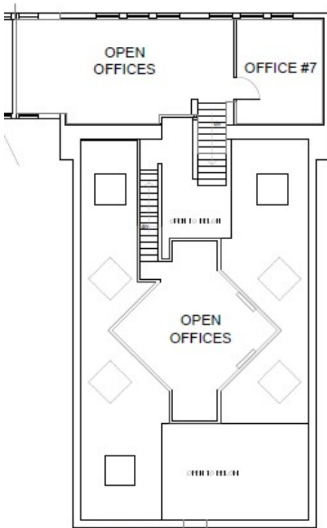
② SUITE 112 UPPER FLOOR PLAN
